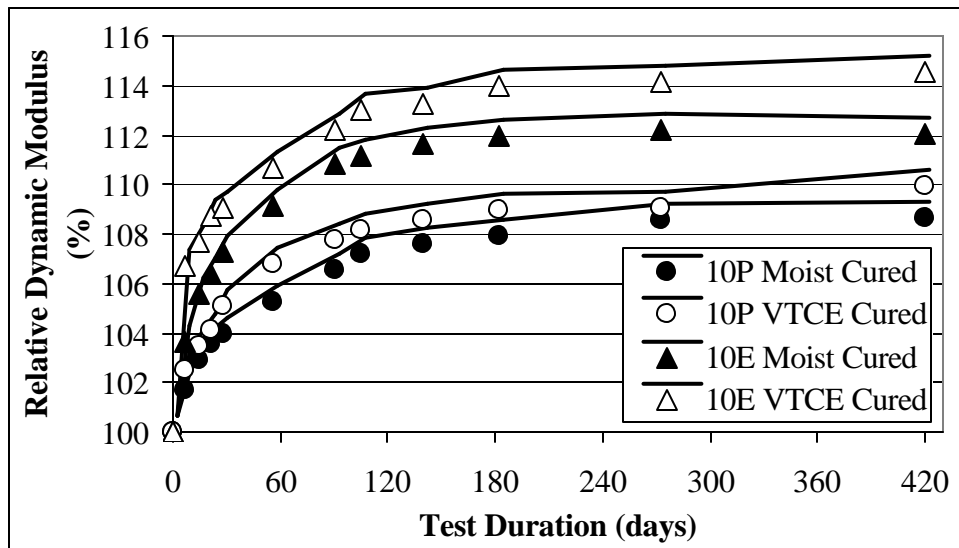
Fig. 3. Change in dynamic modulus of concrete due to exposure to sulfate solution.
