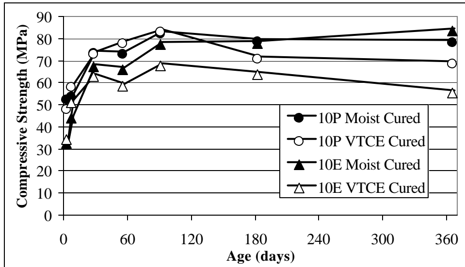
Fig. 2. Compressive strength of concrete mixtures.
